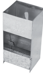
Tolvilla Especial machos Rabbit feeder males 1 hole Cod. 11315 + cm: 15 x 14 x 30 h.
