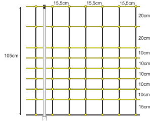
Malla eléctrica cabras 1,05 x 50m Electric mesh for goats 1,05x50m
